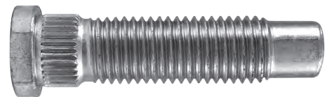
561-492 M12 x 1.5 x 48.3mm Knurl diameter: 12.84mm
