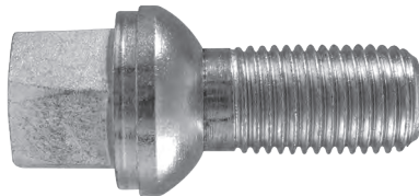
561-467 M14 x 1.5R x 36mm 17mm Hex
