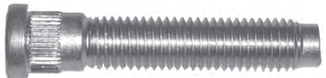
561-424 M14 x 2.0 x 73mm Knurl diameter: 15.78mm
